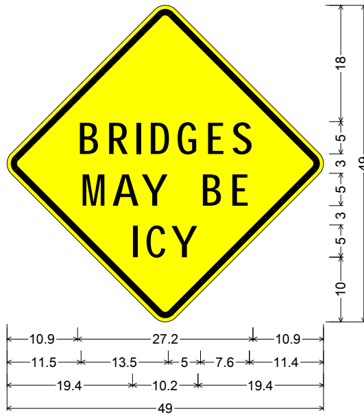
36.0" across sides 2.3" Radius, 0.9" Border, 0.6" Indent, Black on Yellow; "BRIDGES" D; "MAY BE" D; "ICY" D;
