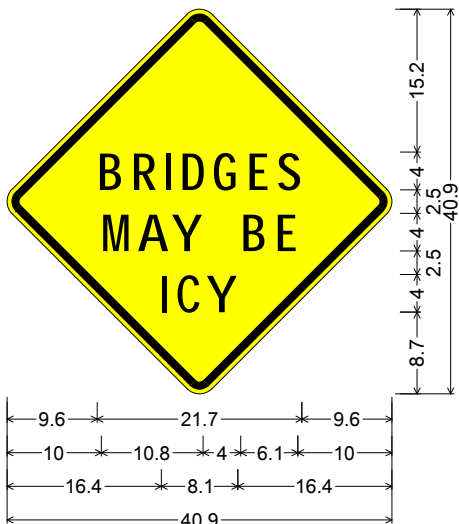
30.0" across sides 1.9" Radius, 0.8" Border, 0.5" Indent, Black on Yellow; "BRIDGES" D; "MAY BE" D; "ICY" D;
