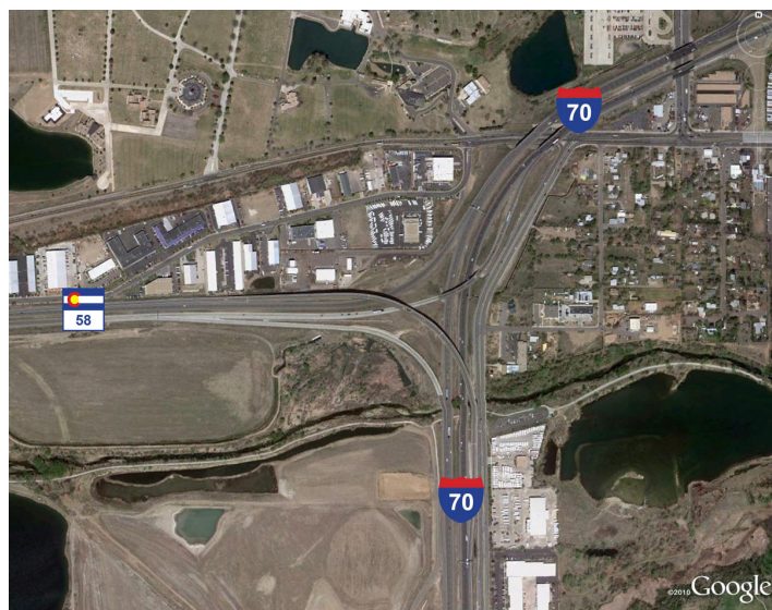
Figure 2-14. Three-Leg Version of Diamond Interchange with Flyover Ramp
