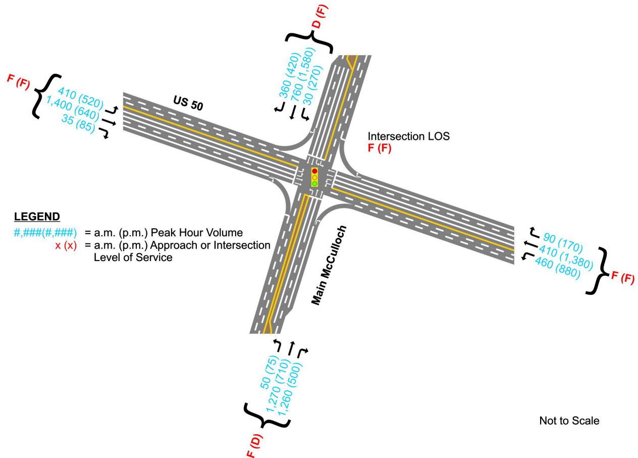
Figure 1-10. 2035 Traffic Patterns at US 50 and Main McCulloch Blvd.
