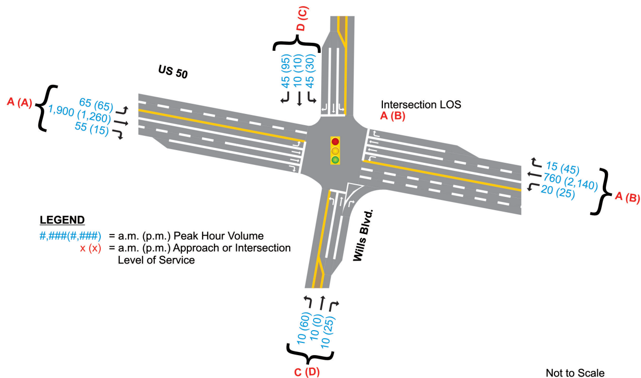
Figure 1-17. Schematic of US 50 and Wills Blvd. with 2011 Travel Patterns
