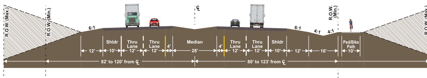
Figure 2-3. Cross Section of the Four-Lane US 50 Option
