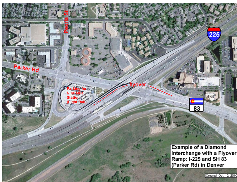
Figure 2-13. Aerial Photo of a Diamond Interchange with Flyover Ramp at I-225 and SH 83 in Denver
