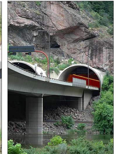
E | Flare tunnel portals and extend them out from the rock cut face.
