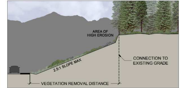
Typical methods deliver an engineered slope poorly integrated into existing grade.
