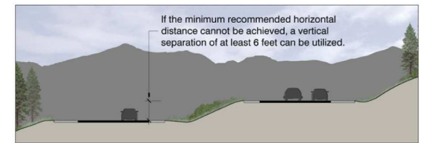
D | Vertical separation can be accomplished through structured or embankment solutions, or a combination of both.
