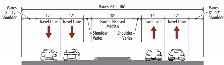
Four General Purpose Lanes 64th Parkway to CO 170
