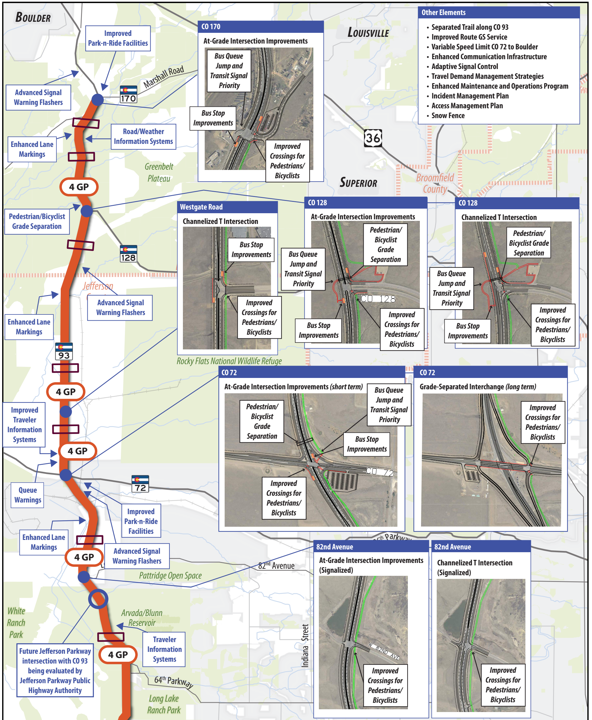
Four General Purpose Lanes 64th Parkway to CO 170
