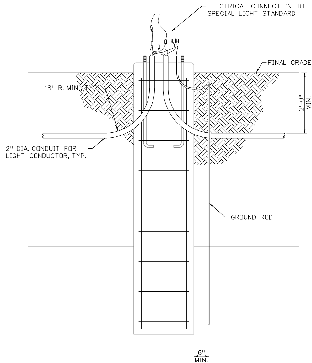
DRILLED CAISSON FOUNDATION ELECTRICAL CONFIGURATION
