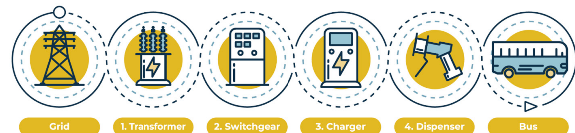
Figure 6: Typical Battery Electric Bus Charging Station Schematic 44
