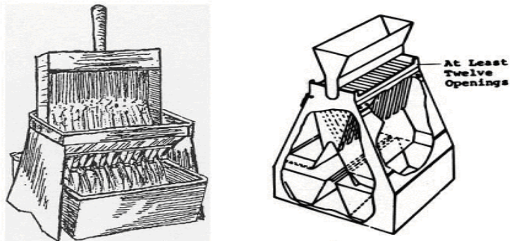
(b) Small Sample Splitters For Fine Aggregate
