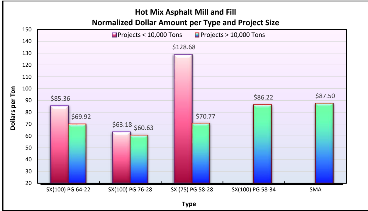
Figure 13.64 HMA Mill and Fill Normalized Dollar per Product Type
