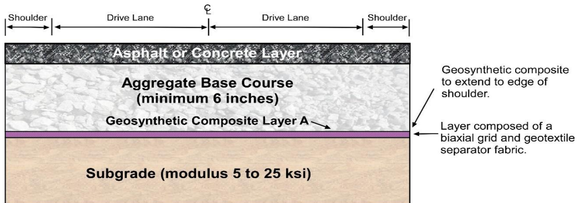
Figure I.1 Typical Section
