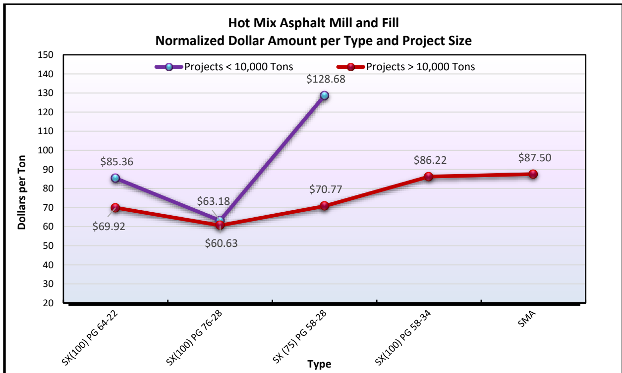
Figure 13.63 HMA Mill and Fill Normalized Dollar per Product Type
