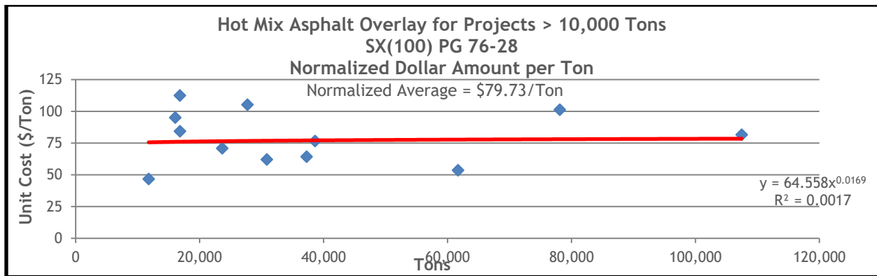
Figure 13.61 HMA Overlay Normalized Unit Costs for SX(100) PG 76-28 on Projects Greater Than 10,000 Tons
