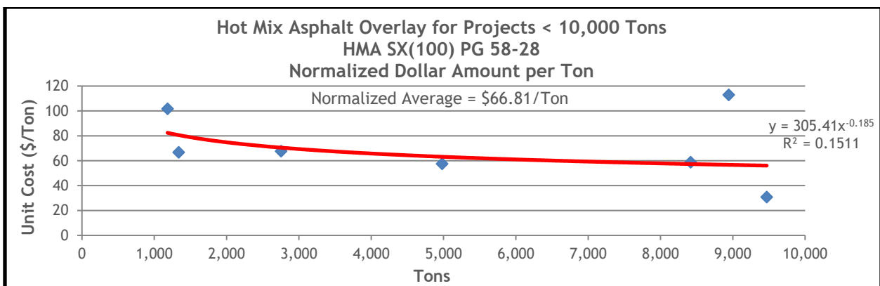
Figure 13.53 HMA Overlay Normalized Unit Costs for SX(100) PG 58-28 on Projects Less Than 10,000 Tons
