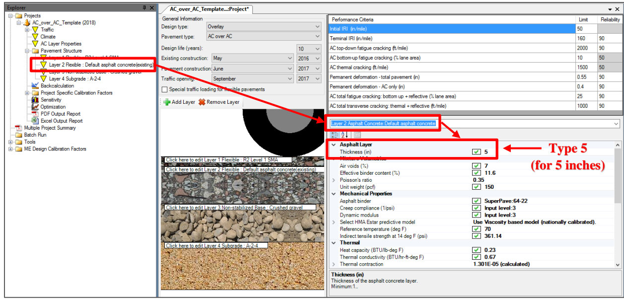
Figure 8.53 Existing Layer Thickness if Milling is Planned
