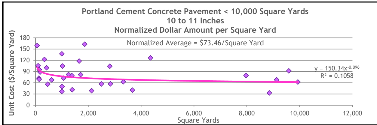
Figure 13.38 PCCP Normalized Dollar Amount for Projects of 10 to 11 Inches in Thickness and Less Than 10,000 Square Yards in Size
