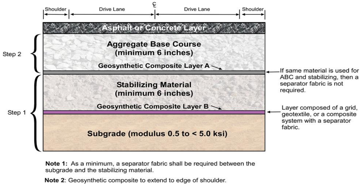
Figure I.2 Two Step Process to Stabilize Soft Subgrade Materials
