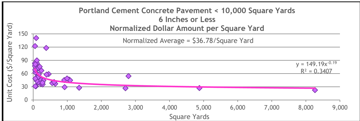
Figure 13.35 PCCP Normalized Dollar Amount for Projects of 6 Inches or Less in Thickness and Less Than 10,000 Square Yards in Size
