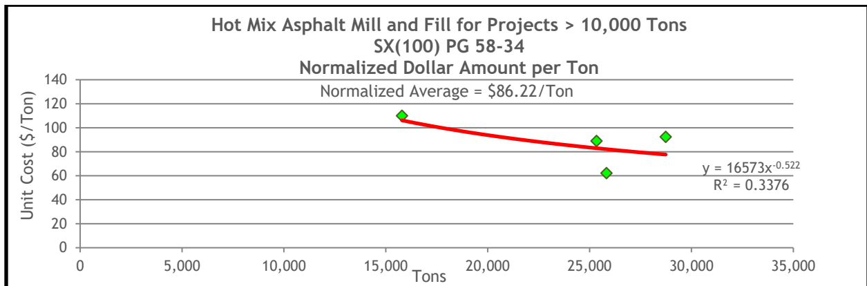
Figure 13.74 HMA Mill and Fill Normalized Unit Costs for SX(100) PG 58-34 on Projects Greater Than 10,000 Tons
