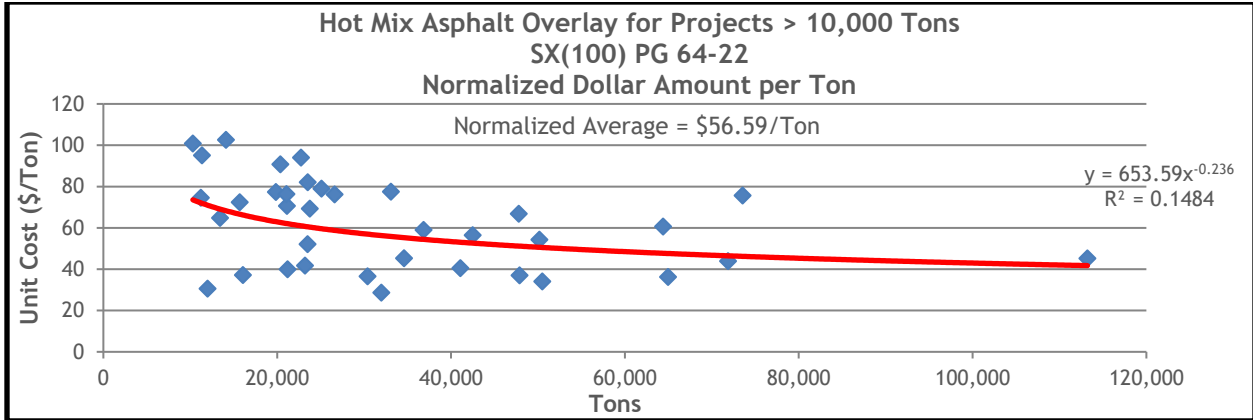
Figure 13.57 HMA Overlay Normalized Unit Costs for SX(100) PG 64-22 on Projects Greater Than 10,000 Tons
