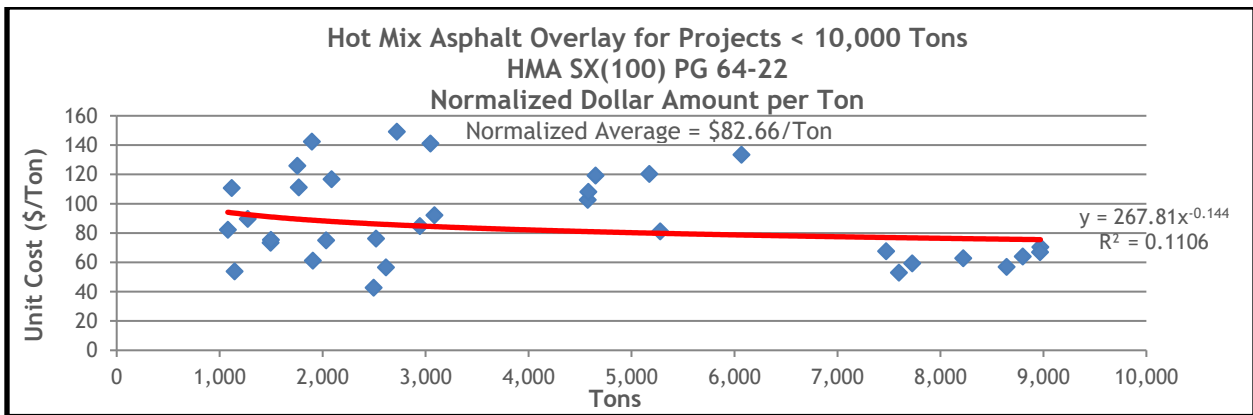
Figure 13.52 HMA Overlay Normalized Unit Costs for SX(100) PG 64-22 on Projects Less Than 10,000 Tons
