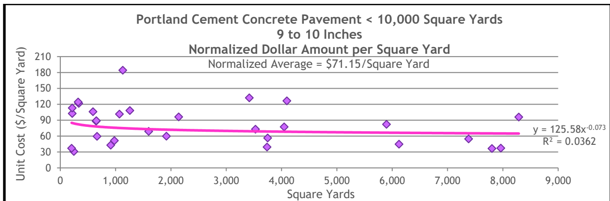
Figure 13.37 Normalized Dollar Amount for Projects of 9 to 10 Inches in Thickness and Less Than 10,000 Square Yards in Size
