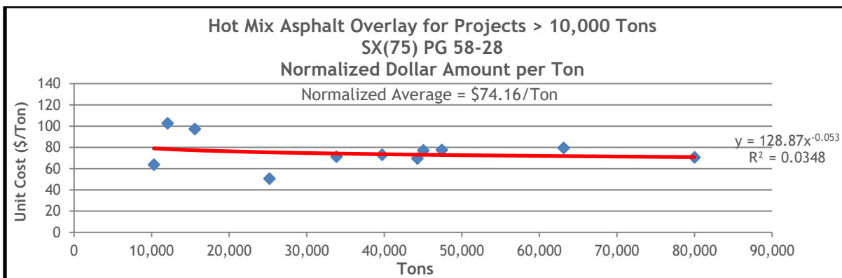
Figure 13.59 HMA Overlay Normalized Unit Costs for SX(100) PG 58-28 on Projects Greater Than 10,000 Tons
