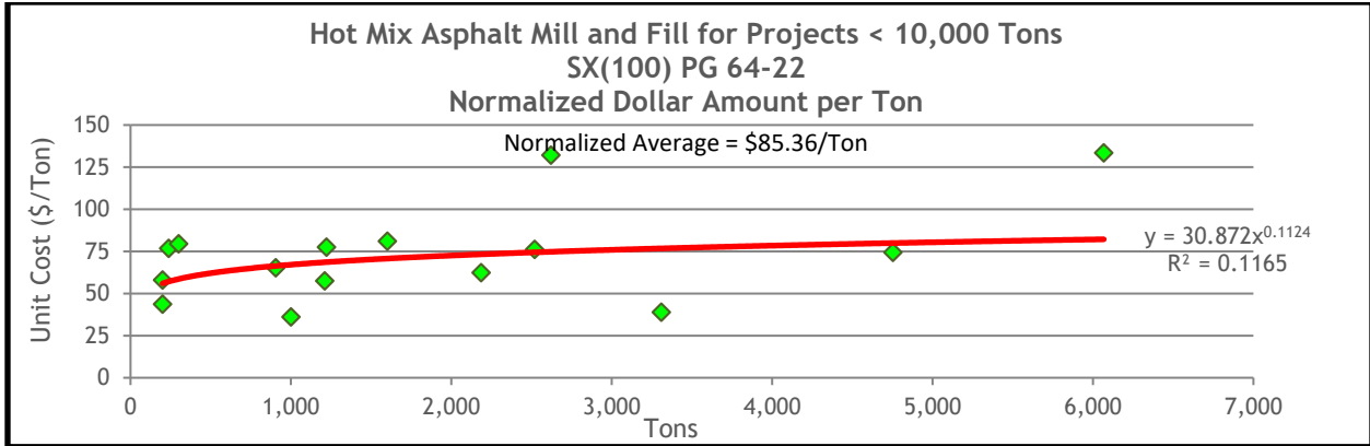
Figure 13.66 HMA Mill and Fill Normalized Unit Costs for SX(100) PG 64-22 on Projects Less Than 10,000 Tons
