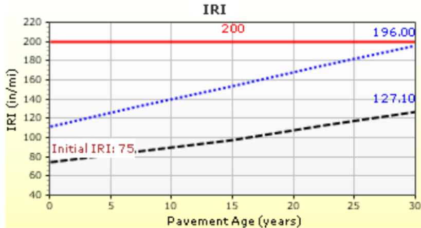
Figure 13.5 IRI at 95 Percent Reliability
