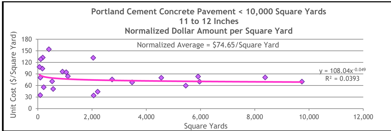
Figure 13.39 PCCP Normalized Dollar Amount for Projects of 11 to 12 Inches in Thickness and Less Than 10,000 Square Yards in Size
