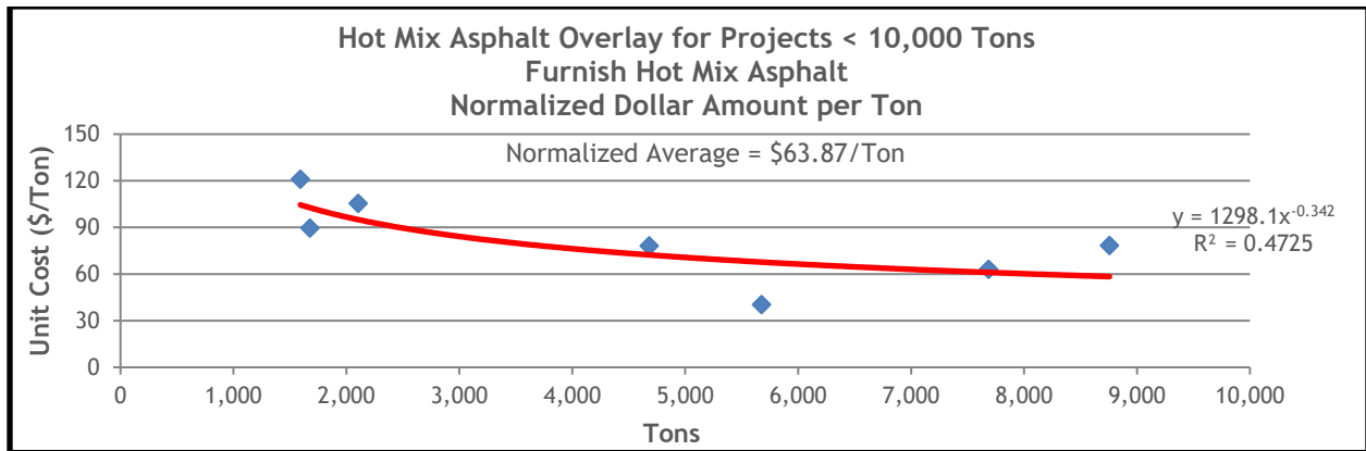
Figure 13.55 HMA Overlay Normalized Unit Costs for Furnish HMA on Projects Less Than 10,000 Tons
