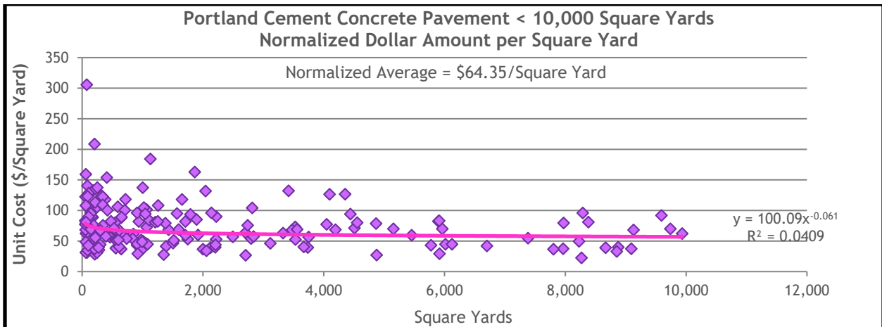
Figure 13.34 PCCP Normalized Dollar Amount per Total Square Yards for Projects Less Than 10,000 Square Yards
