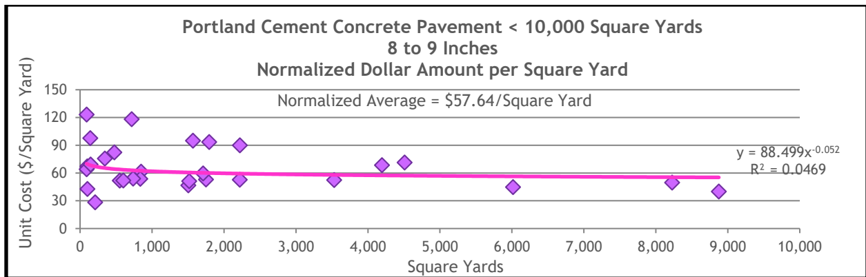
Figure 13.36 Normalized Dollar Amount for Projects of 8 to 9 Inches in Thickness and Less Than 10,000 Square Yards in Size
