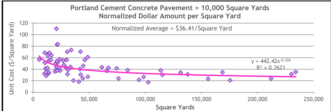
Figure 13.41 PCCP Normalized Dollar Amount per Total Square Yards for Projects Greater Than 10,000 Square Yards
