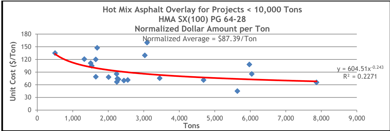
Figure 13.51 HMA Overlay Normalized Unit Costs for SX(100) PG 64-28 on Projects Less Than 10,000 Tons
