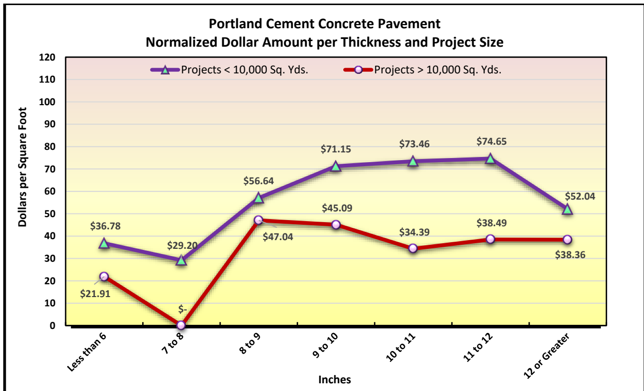
Figure 13.32 PCCP Normalized Dollar Amount per Thickness
