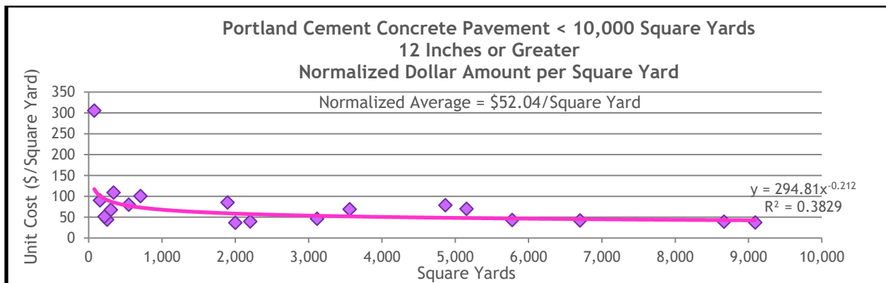
Figure 13.40 PCCP Normalized Dollar Amount for Projects of 12 Inches or Greater in Thickness and Less Than 10,000 Square Yards in Size
