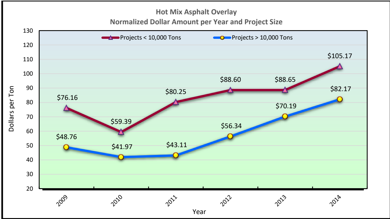
Figure 13.47 HMA Overlay Normalized Dollar per Year and Project Size
