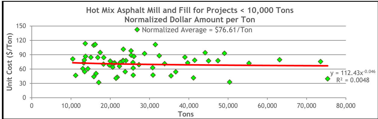
Figure 13.65 HMA Mill and Fill Normalized Unit Costs for Projects Less Than 10,000 Tons
