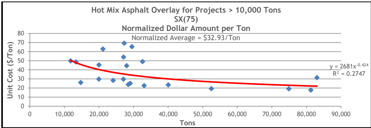
Figure 13.58 HMA Overlay Normalized Unit Costs for SX(75) on Projects Greater Than 10,000 Tons
