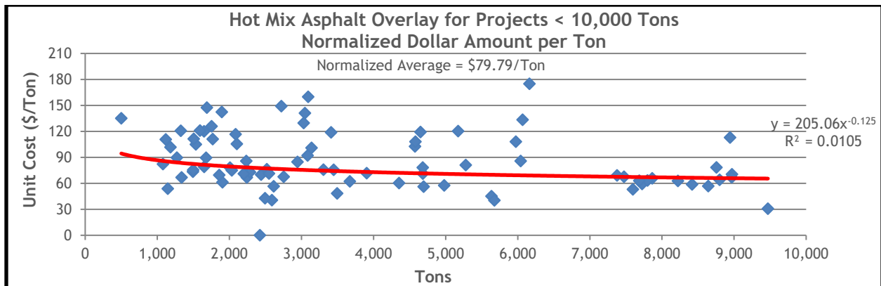
Figure 13.50 HMA Overlay Normalized Dollar Amount for Projects Less Than 10,000 Tons
