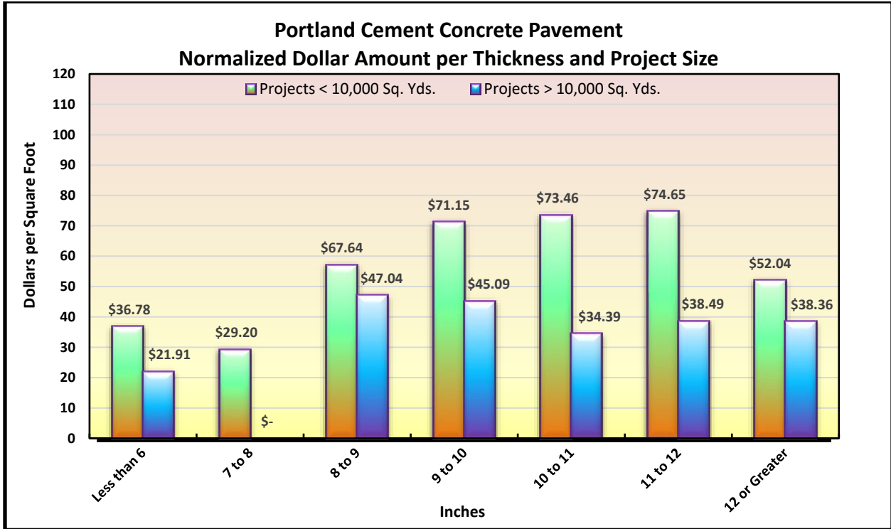
Figure 13.33 PCCP Normalized Dollar Amount per Thickness
