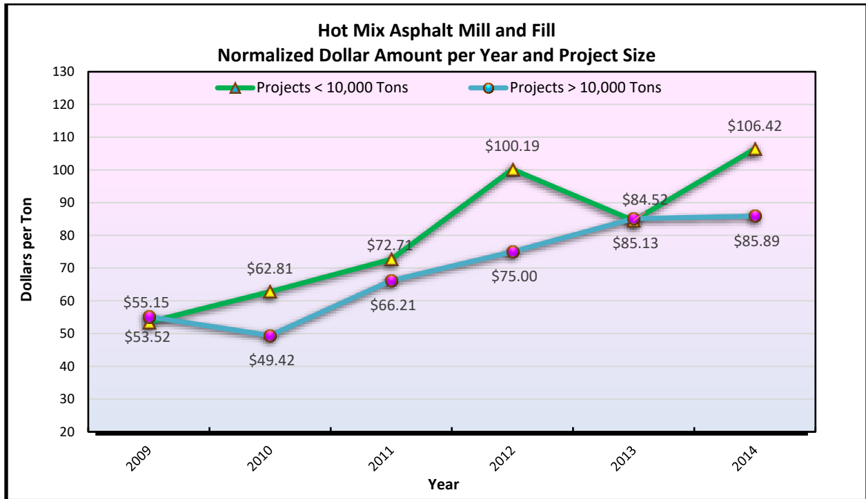
Figure 13.62 HMA Mill and Fill Normalized Dollar per Year and Project Size
