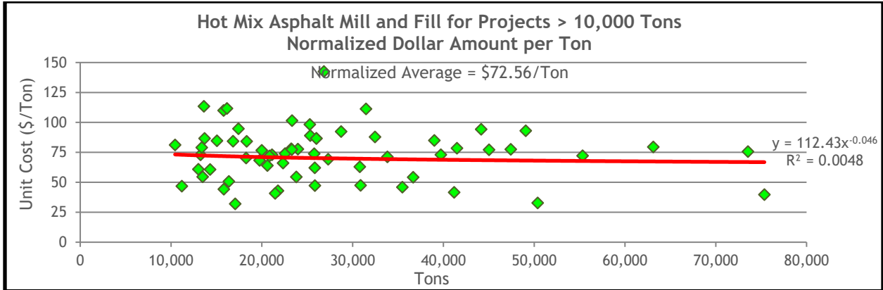
Figure 13.69 HMA Mill and Fill Normalized Unit Costs for Projects Greater Than 10,000 Tons
