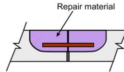
Figure 10.15 Typical Dowel Bar Retrofit Sequencing of the Installation From Figure 4-9.7, Construction Procedures for Retrofitted Dowel Bar Installation Techniques for Pavement Rehabilitation 1998 (6)
