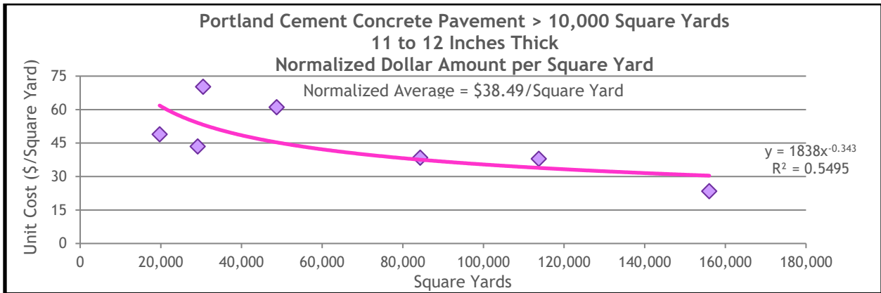
Figure 13.45 PCCP Normalized Dollar Amount for Projects of 11 to 12 Inches in Thickness and Greater Than 10,000 Square Yards in Size
