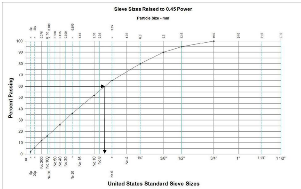
Figure S.2 Gradation Plot
