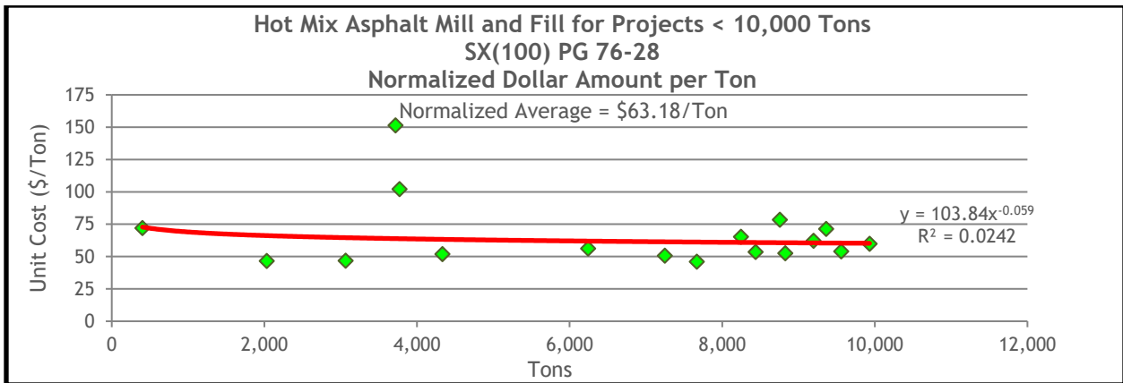
Figure 13.67 HMA Mill and Fill Normalized Unit Costs for SX(100) PG 76-28 on Projects Less Than 10,000 Tons
