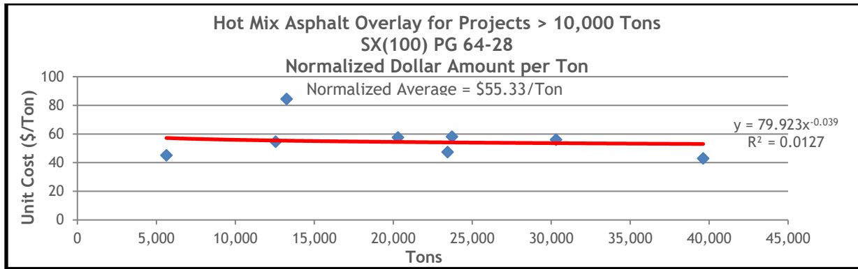
Figure 13.60 HMA Overlay Normalized Unit Costs for SX(100) PG 64-28 on Projects Greater Than 10,000 Tons
