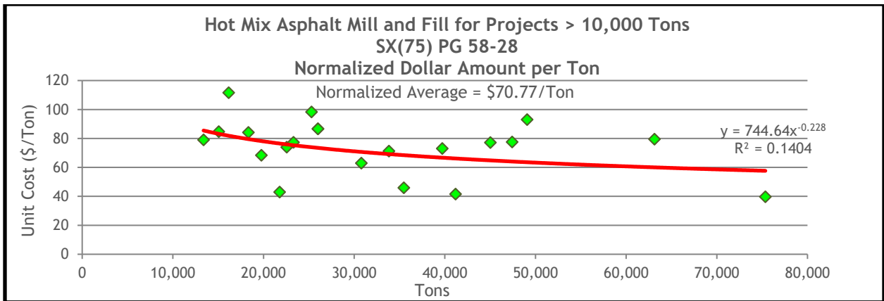
Figure 13.71 HMA Mill and Fill Normalized Unit Costs for SX(100) PG 64-22 on Projects Greater Than 10,000 Tons
