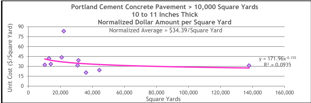
Figure 13.44 Normalized Dollar Amount for Projects of 10 to 11 Inches in Thickness and Greater Than 10,000 Square Yards in Size
