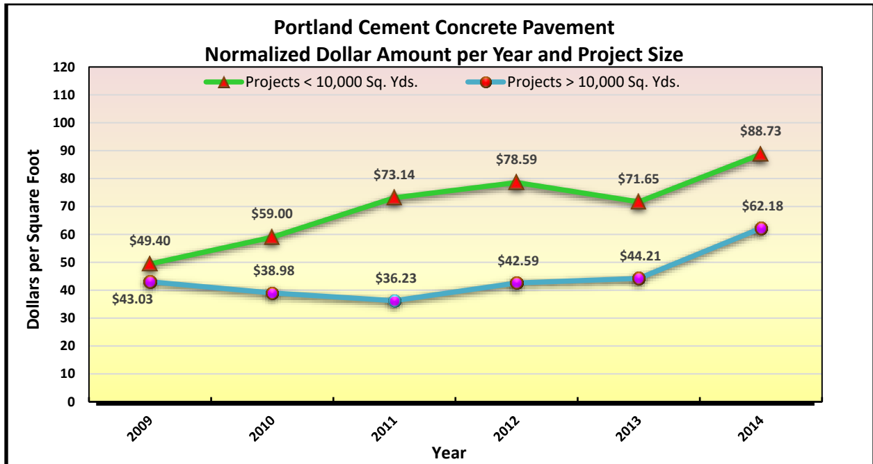
Figure 13.31 PCCP Normalized Dollar Amount per Year
