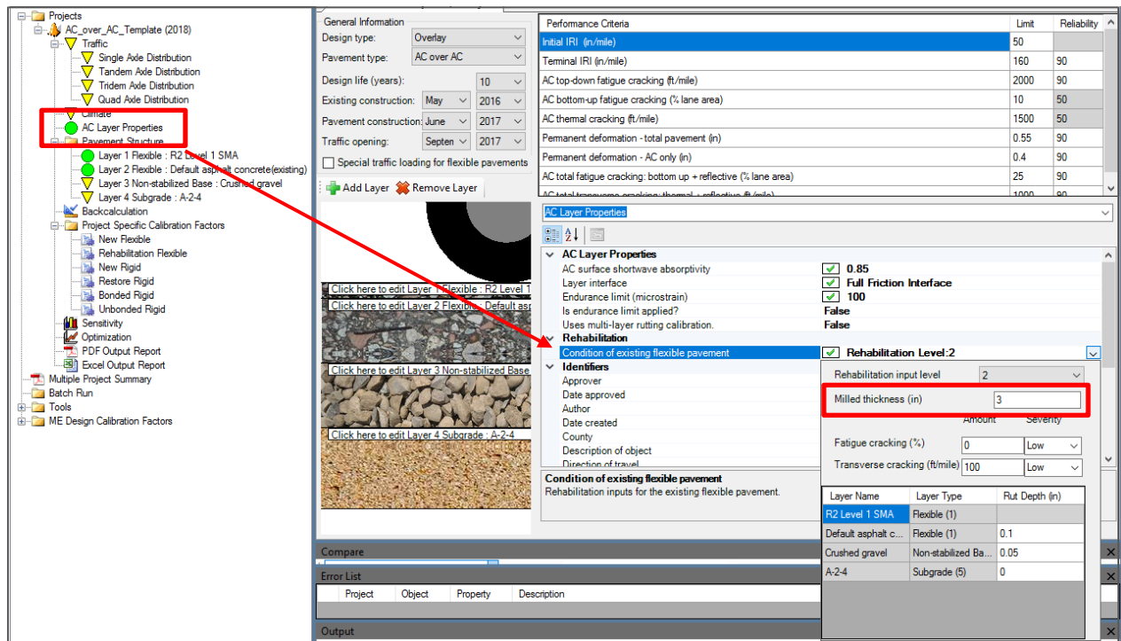
Figure 8.52 Milled Thickness Input Screen
