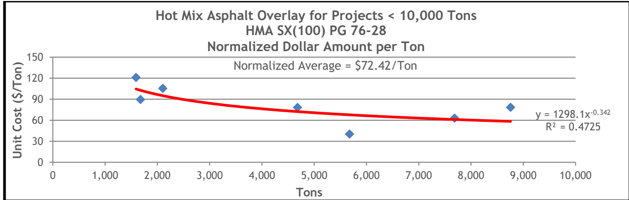
Figure 13.54 HMA Overlay Normalized Unit Costs for SX(100) PG 76-28 on Projects Less Than 10,000 Tons
