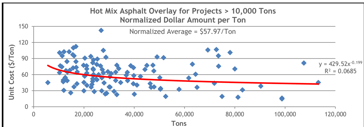
Figure 13.56 HMA Overlay Normalized Unit Costs for Projects with Greater Than 10,000 Tons
