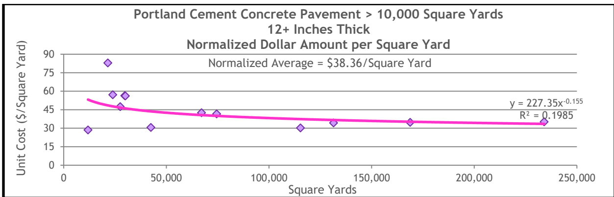
Figure 13.46 PCCP Normalized Dollar Amount for Projects of 12 Inches or Greater in Thickness and Greater Than 10,000 Square Yards in Size
