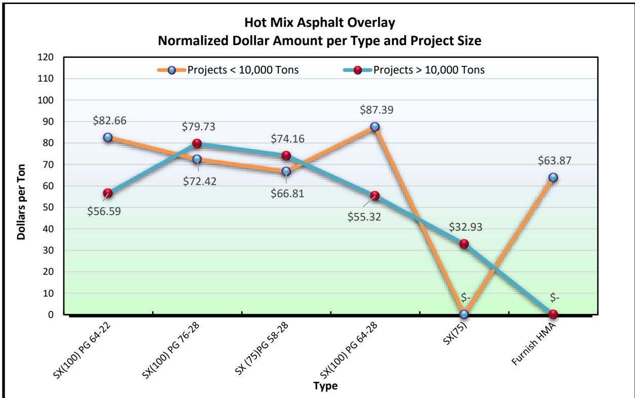
Figure 13.48 HMA Overlay Normalized Dollar per Product Type and Project Size
