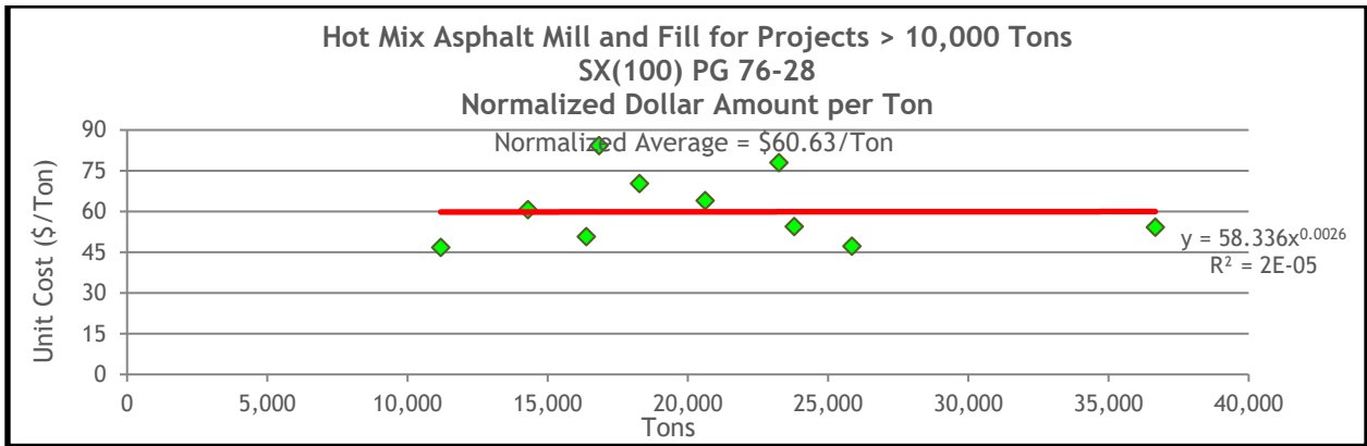
Figure 13.70 HMA Mill and Fill Normalized Unit Costs for SX(100) PG 76-28 on Projects Greater Than 10,000 Tons
