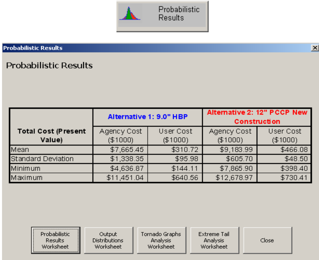
Figure 13.77 Probabilistic Results Screen
