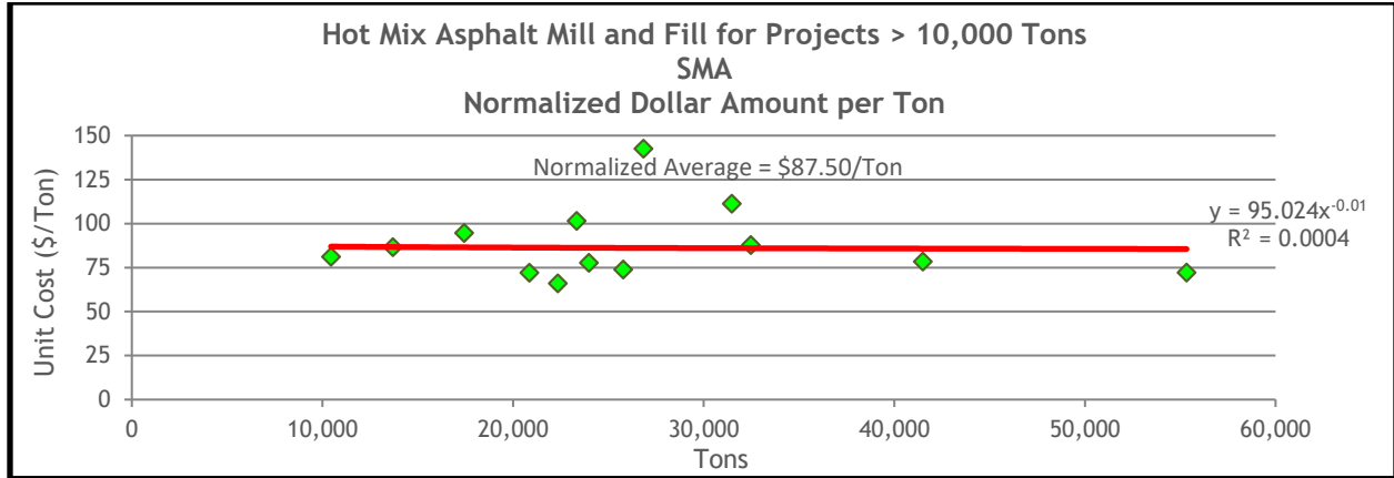
Figure 13.72 HMA Mill and Fill Normalized Unit Costs for SMA on Projects Greater Than 10,000 Tons
