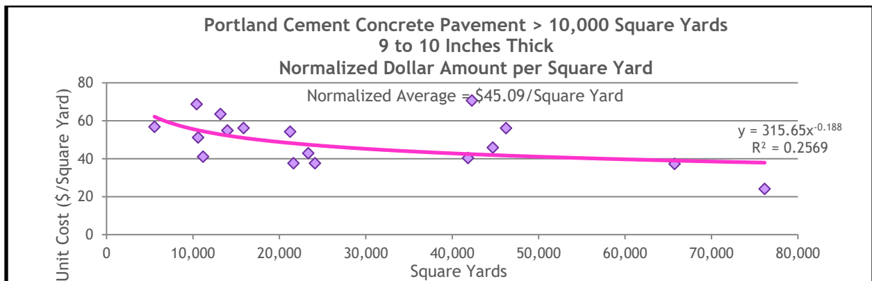
Figure 13.43 PCCP Normalized Dollar Amount for Projects of 9 to 10 Inches in Thickness and Greater Than 10,000 Square Yards in Size
